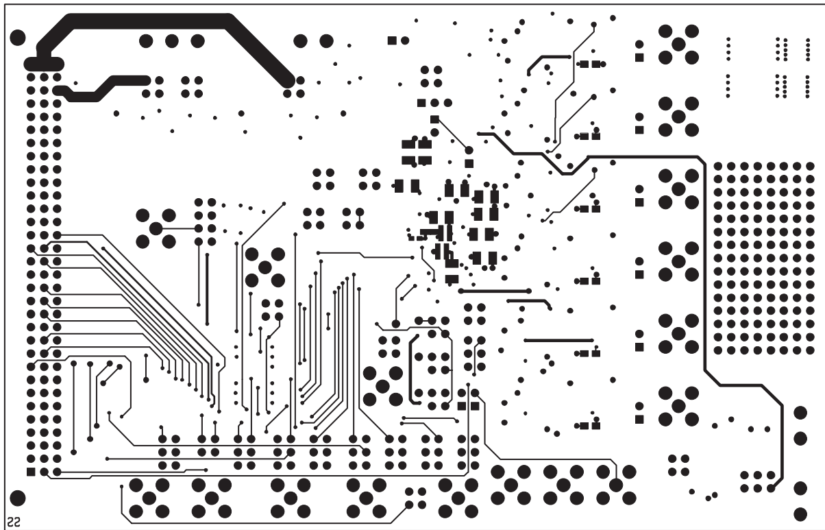
Figure 10. Top Layer Etch
