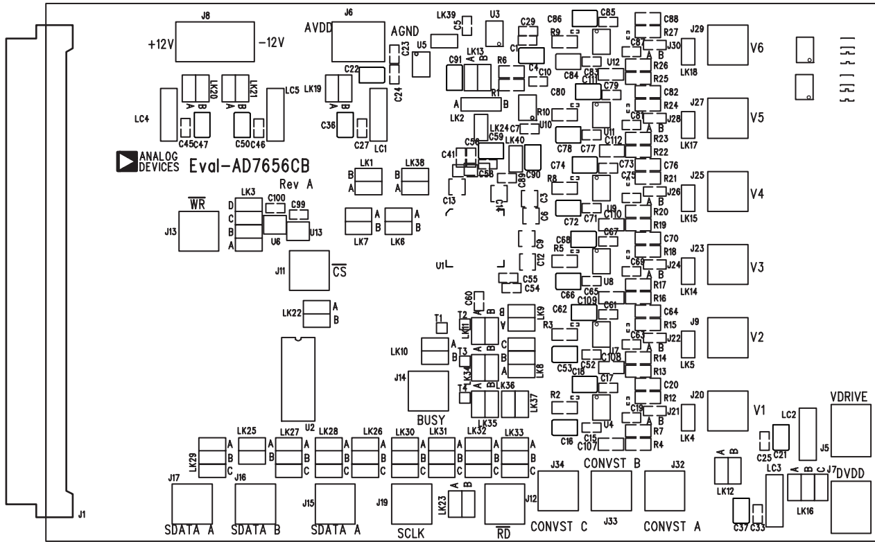
Figure 9. Silkscreen Top Side
